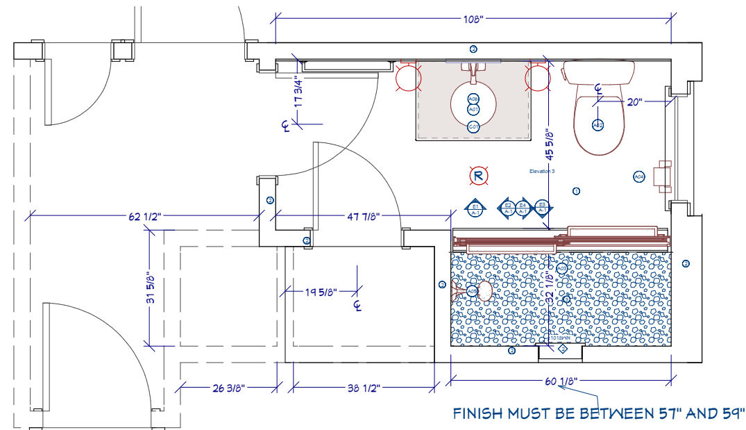
Kitchen and Bath Plan View
