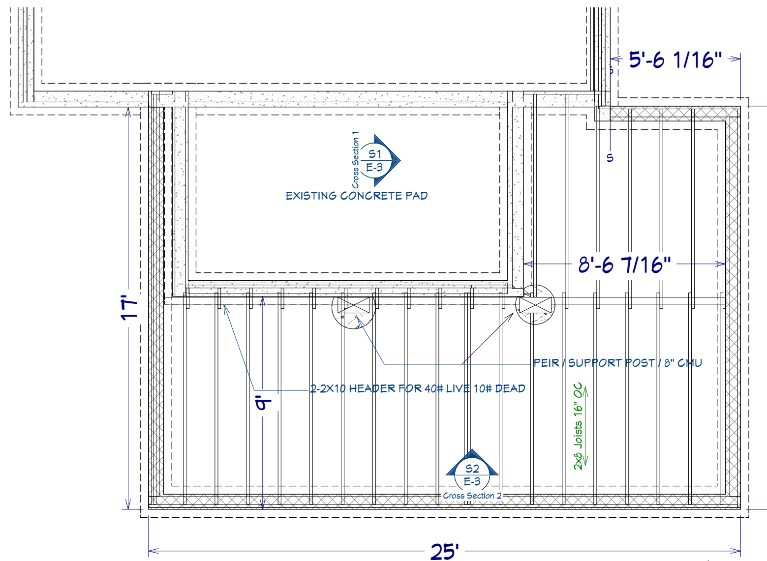
Foundation 1/2 SCALE
