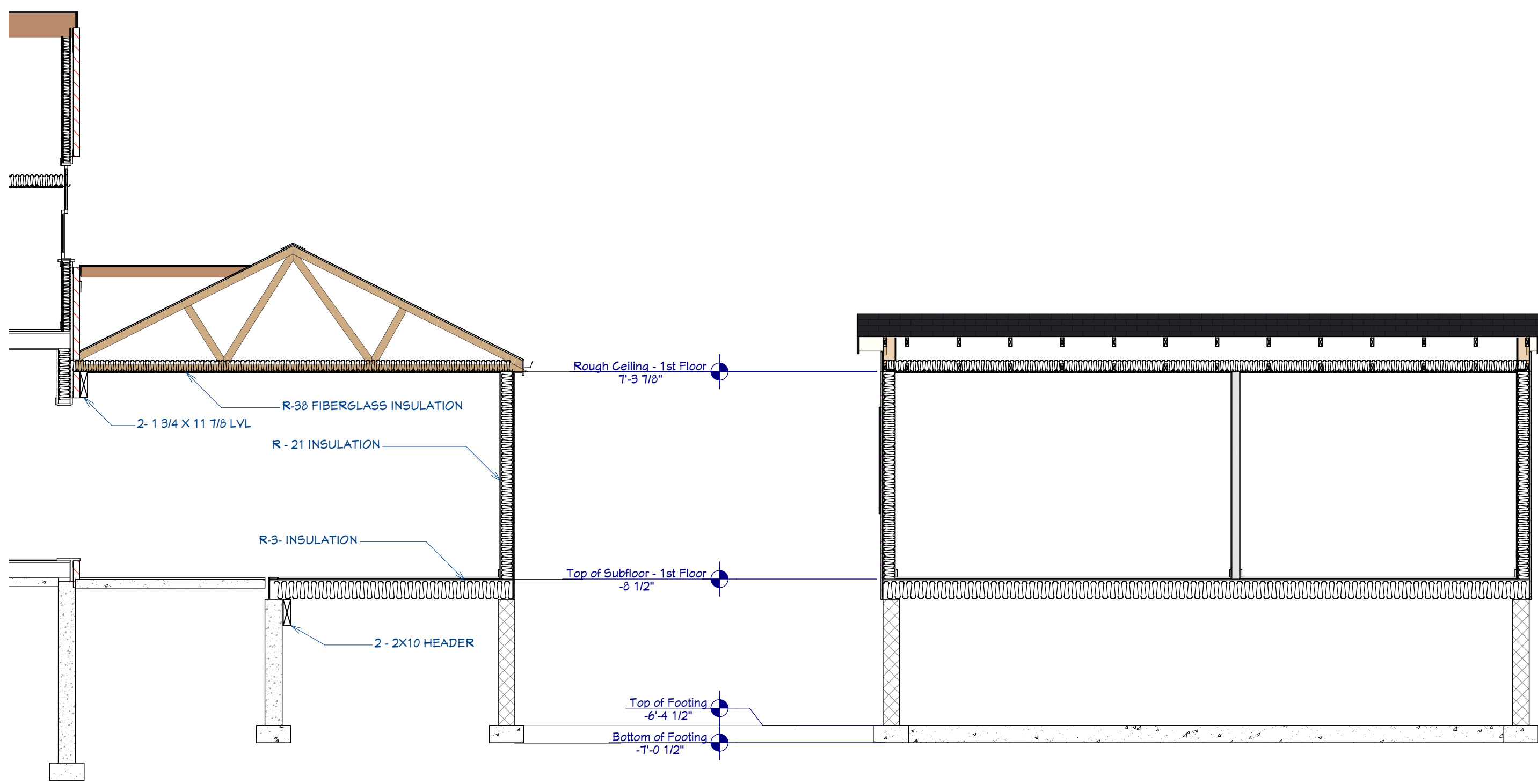
Cross Section 1
